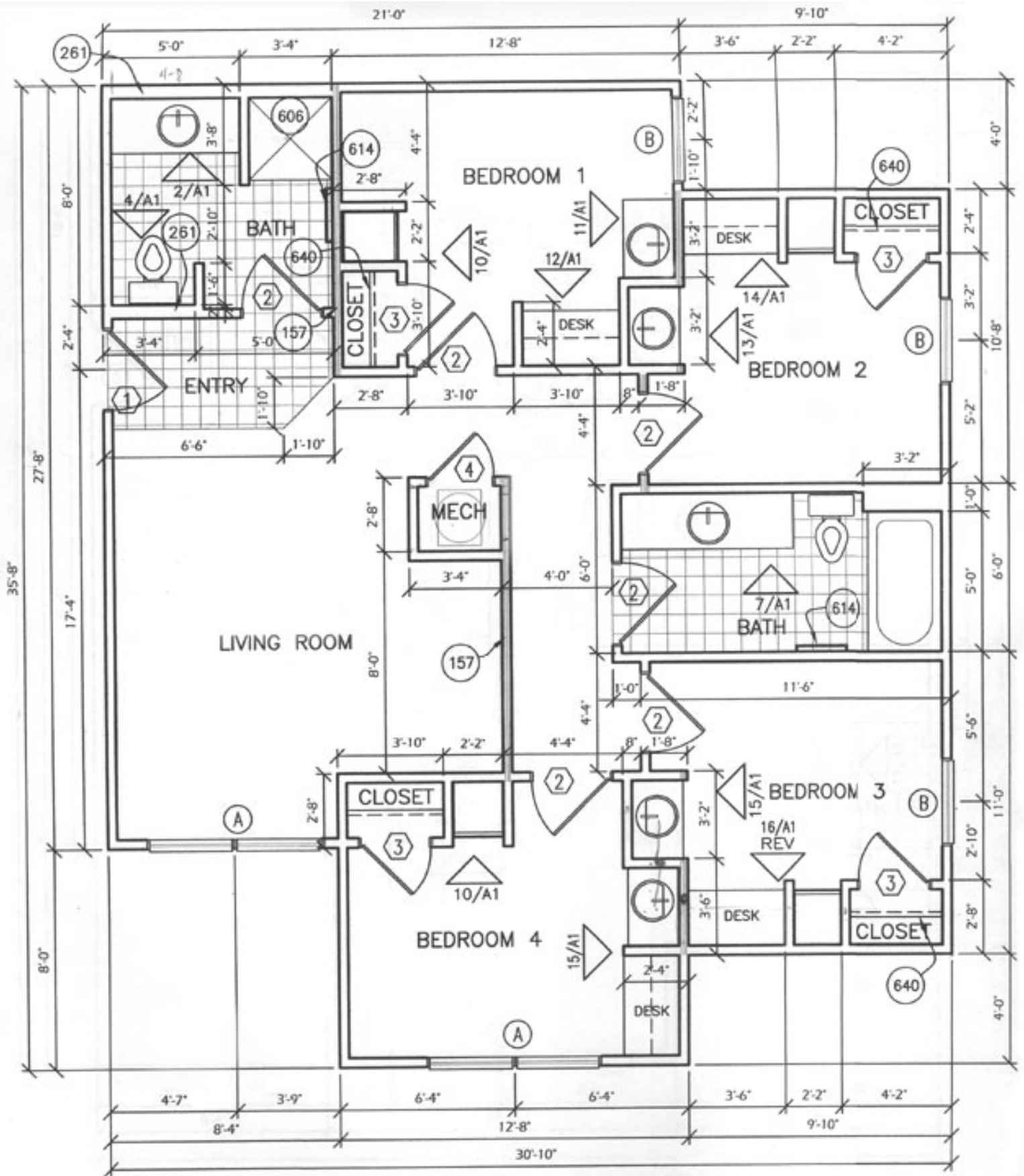
1 TYPICAL UNIT FLOOR PLAN 1/4" = 1'-0"
